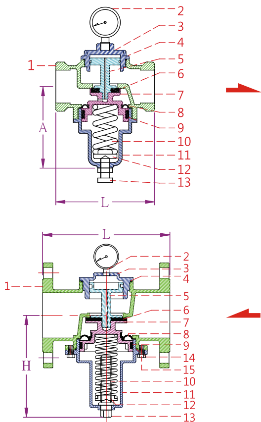
Flow Chart of Direct-Activated Pressure Relief Valve
